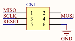
SPI Interface
