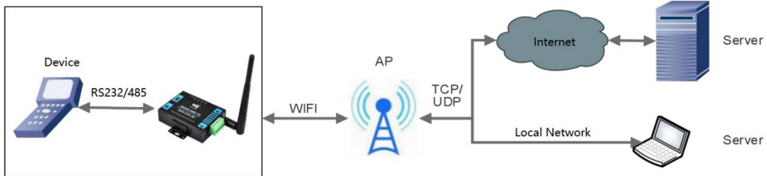
Figure Basic functions of serial server
