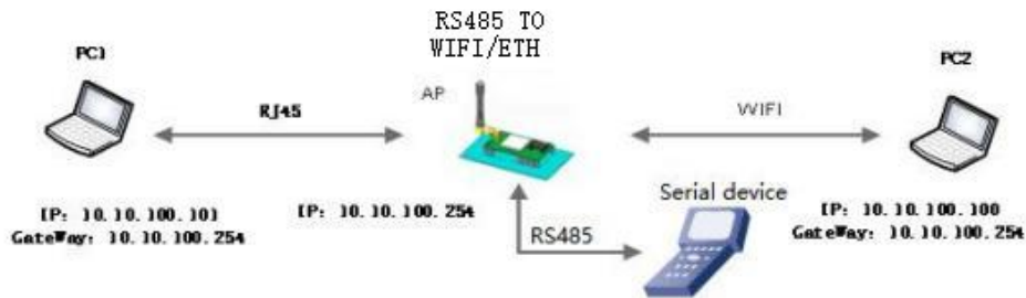
Figure Attached Private Local Area Network (APLAN)
