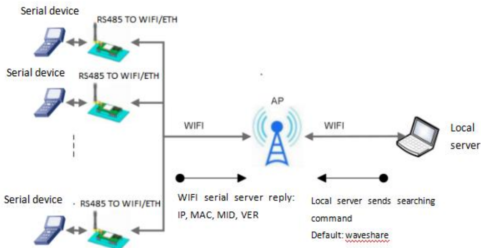
Figure LAN search block diagram
