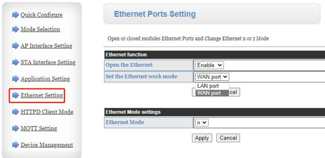
Figure Network Port Mode Setting
