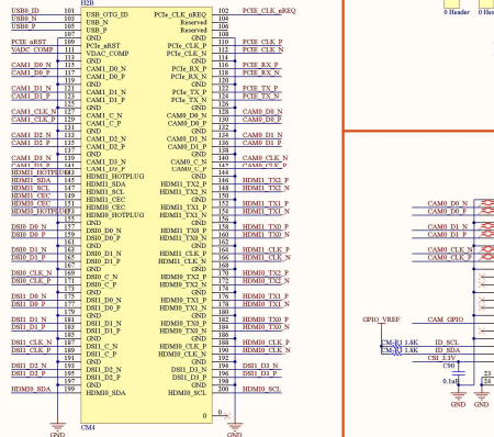
CM4 Interface
