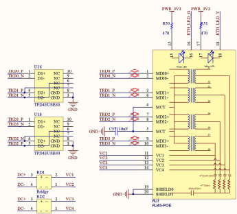
Giga ETH
