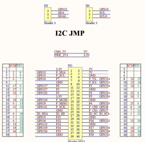
I2C JUMP
