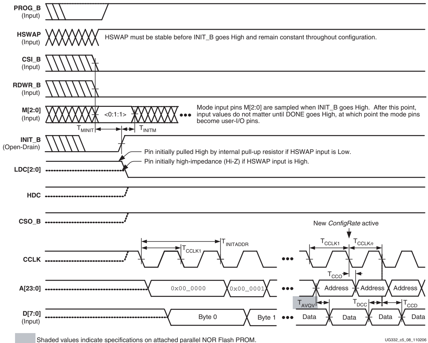
Figure 78: Waveforms for Byte-wide Peripheral Interface (BPI) Configuration (BPI-DN mode shown)
