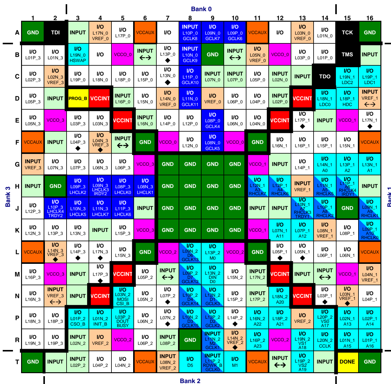
Figure 86: FT256 Package Footprint (top view)
