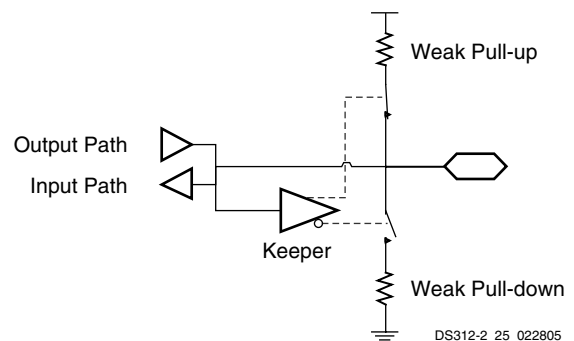
Figure 12: Keeper Circuit
