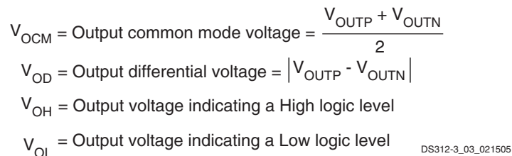
Figure 71: Differential Output Voltages
