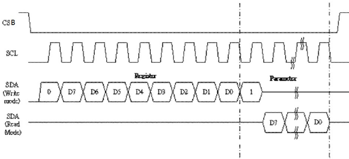
Figure 3.5-3: Read procedure in 3-wire SPI mode
