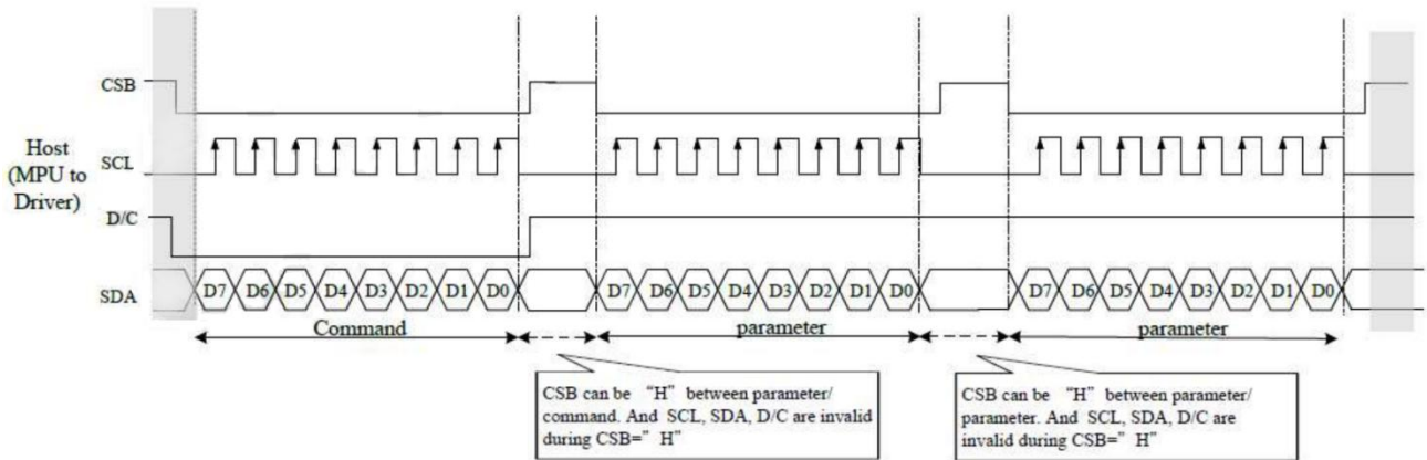
Figure 6-3-1: 4-wire SPI mode
