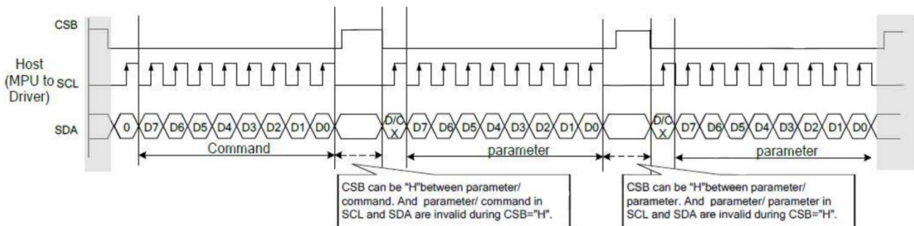
Figure 6-3-2: 3-wire SPI mode
