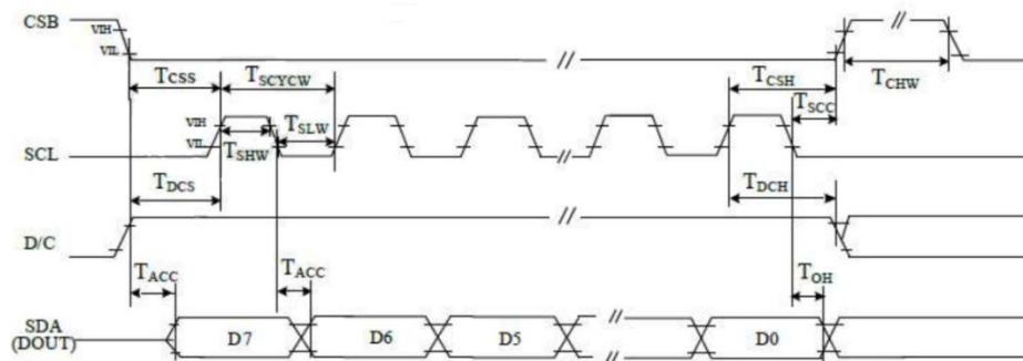
Figure 6-3-3: 4-pin serial interface characteristics
