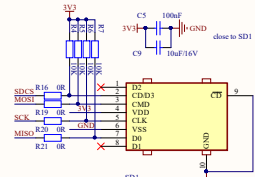
SD-CARD
