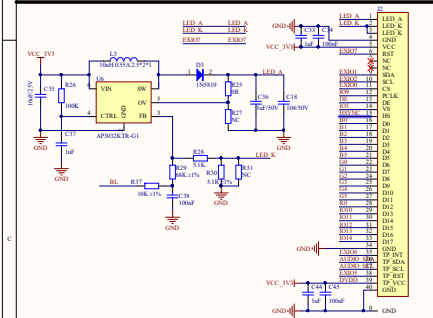
Touch LCD 4inch
