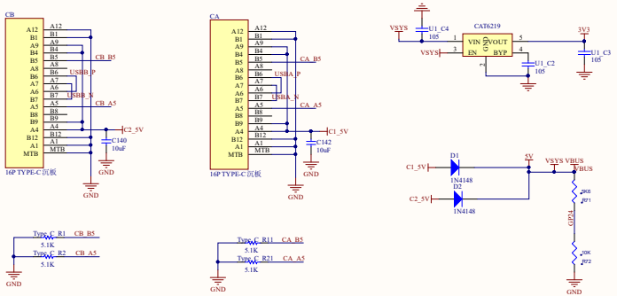
Type C Power
