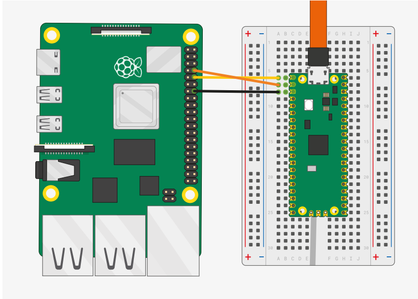
Figure 2. A Raspberry Pi 4 and the Raspberry Pi Pico 2 with UART0 connected together.
