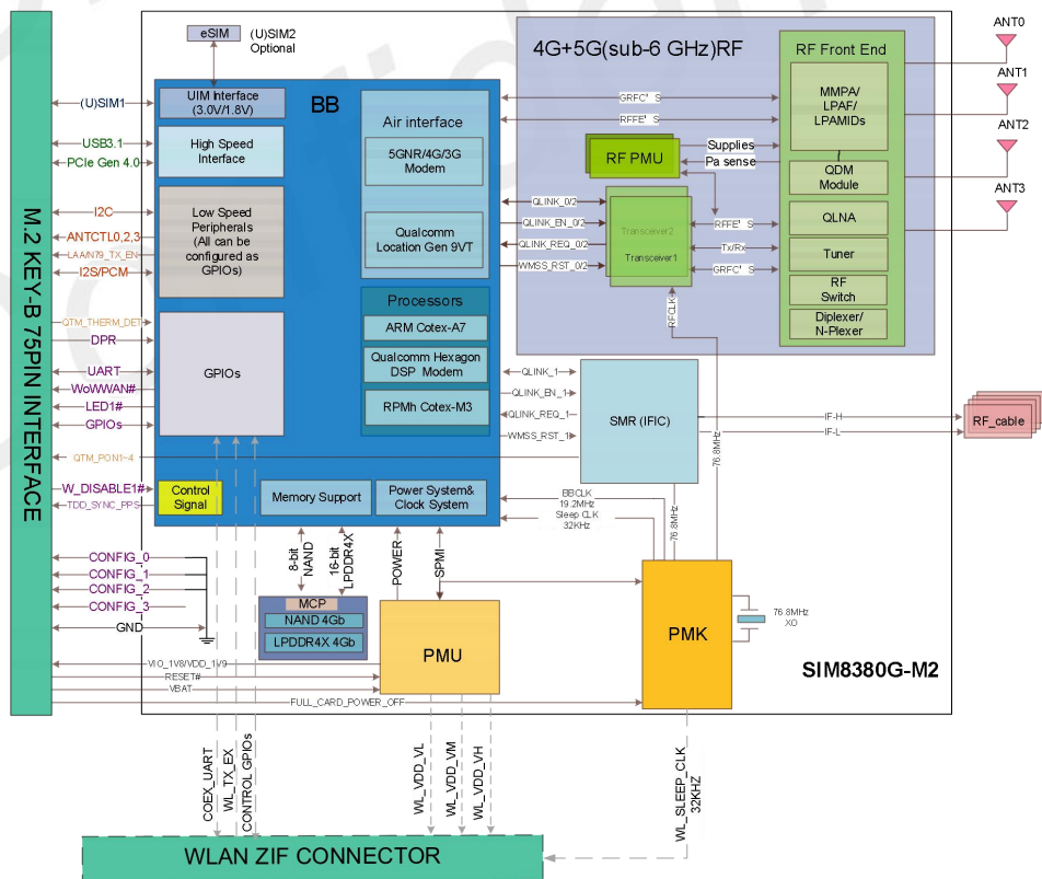
Figure 2: Block diagram
