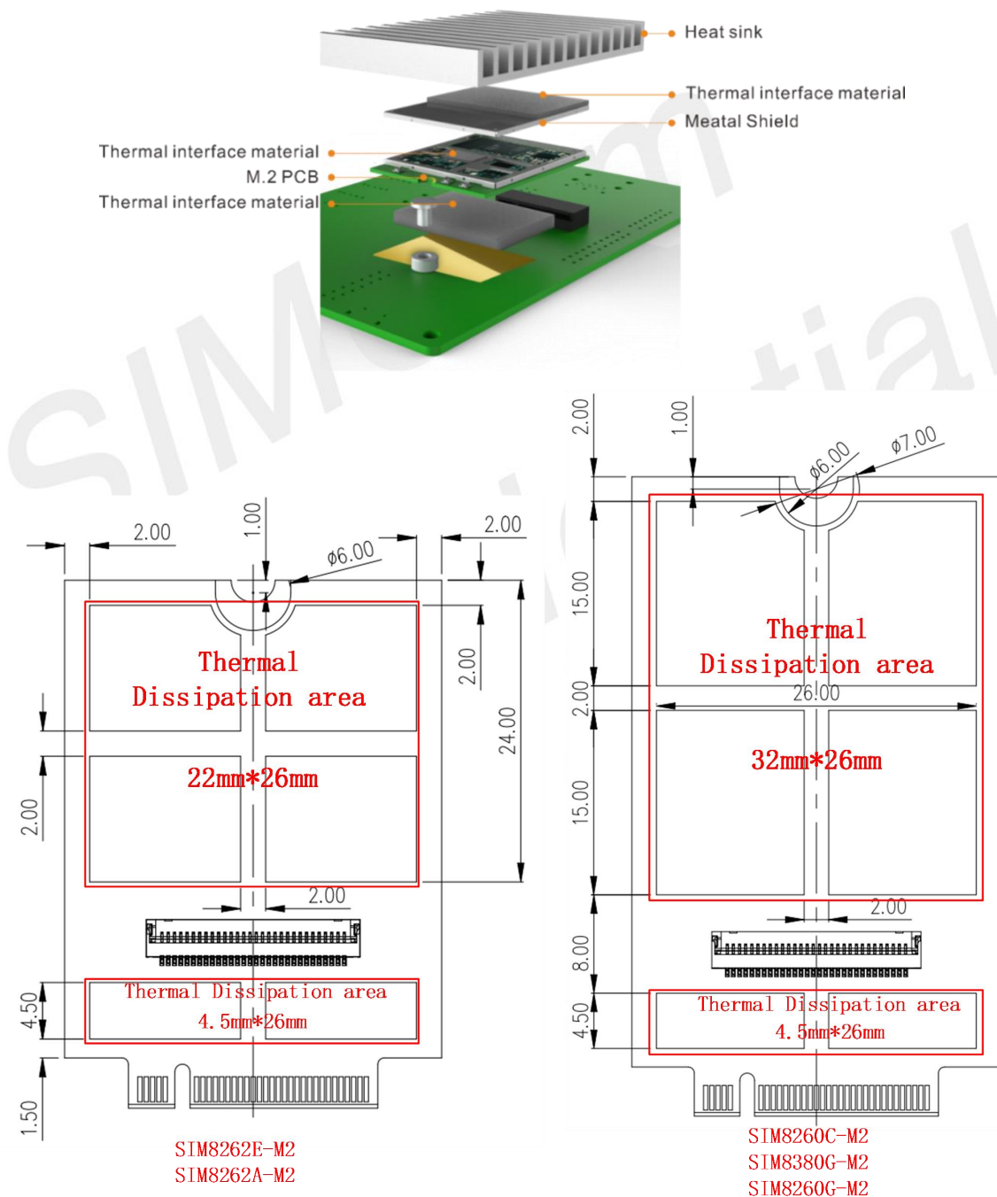
Figure 47: Thermal design diagram
