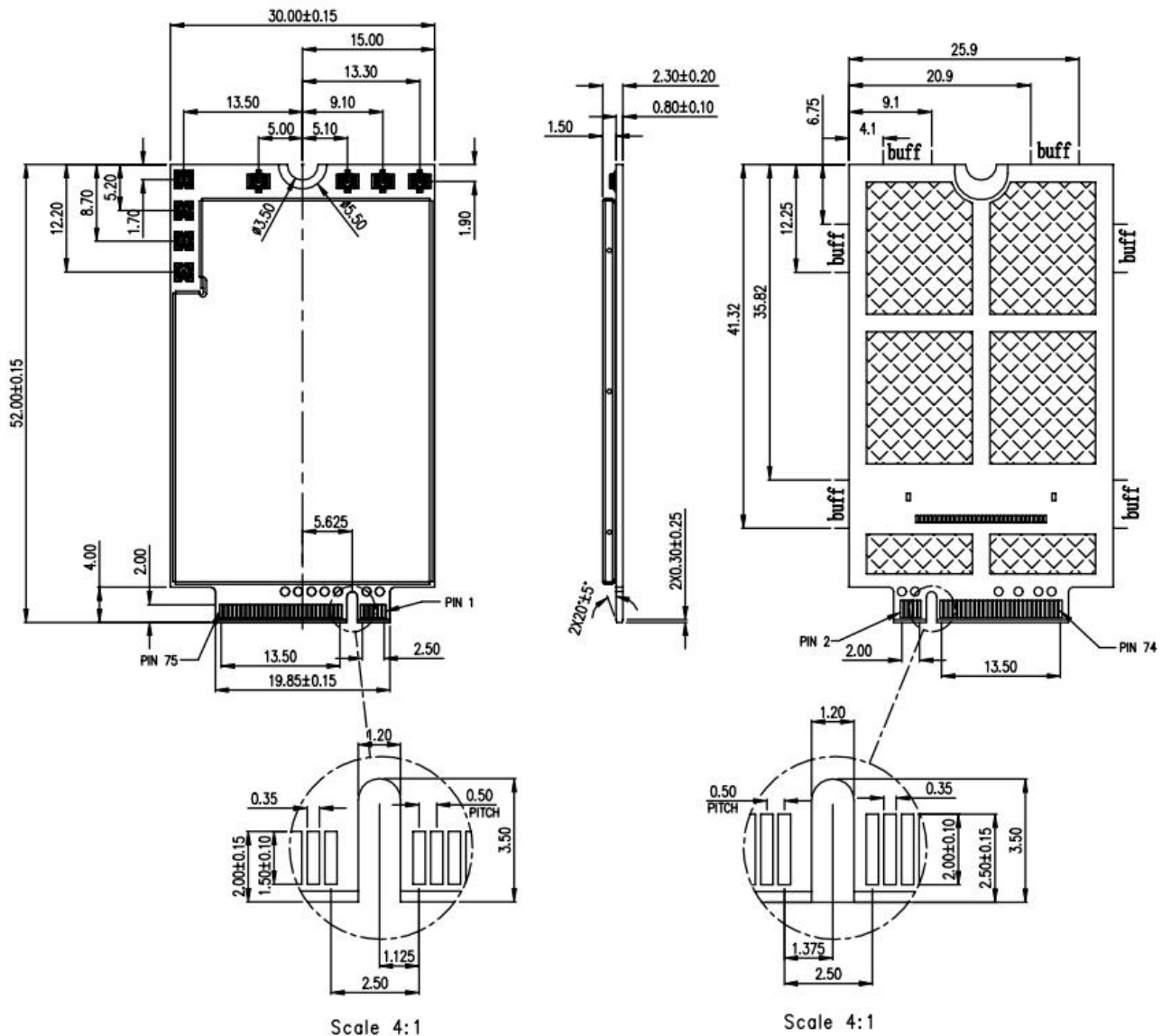
Figure 6: Dimensions of the module (unit: mm)
