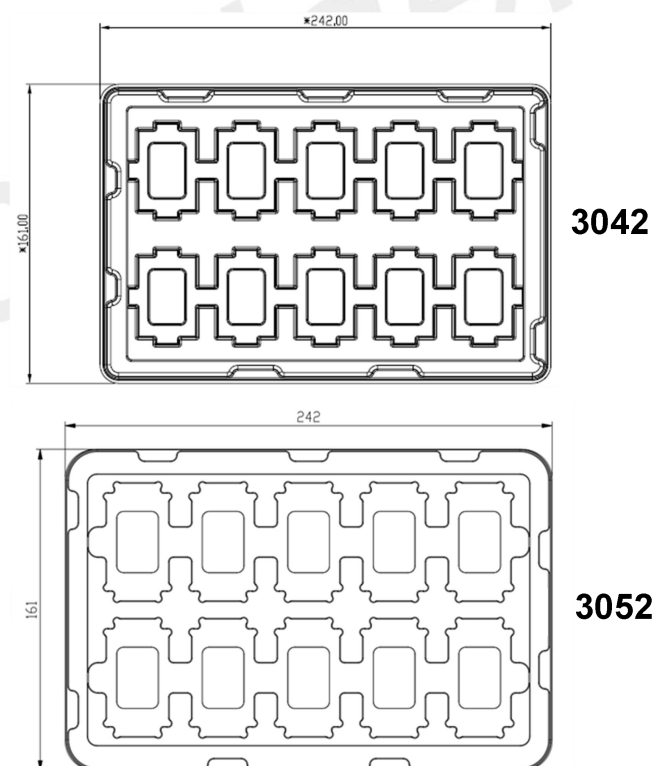
Figure 51: Tray view of the module
