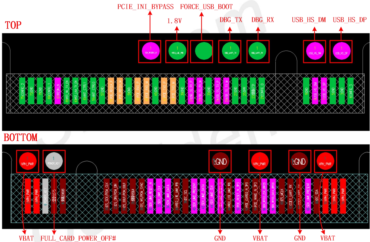
Figure 5: Test point of SIM826XX/SIM8X80-M2 series module
