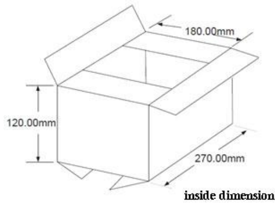
Figure 52: Small carton view
