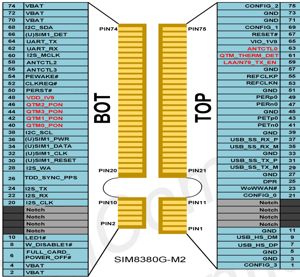
Figure 3: Pin assignment
