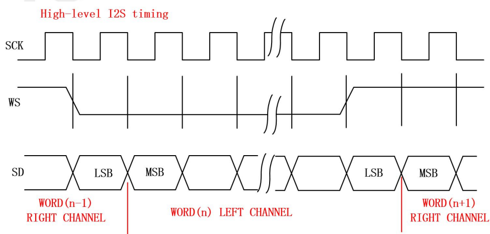
Figure 32: I2S timing
