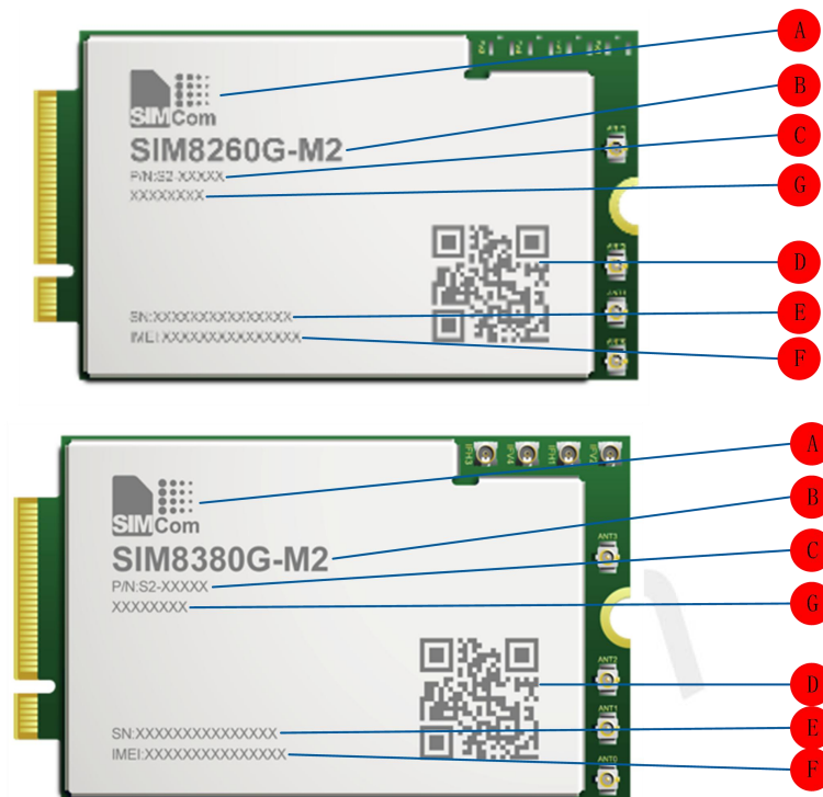
Figure 49: Label description of the module
