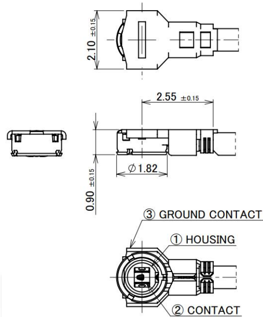
Figure 42: Mechanical information of RF plug
