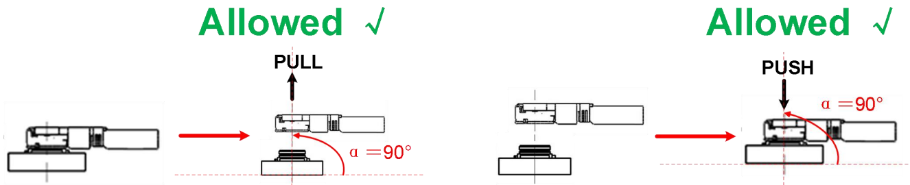
Figure 43: RF cable correct pull and push operation
