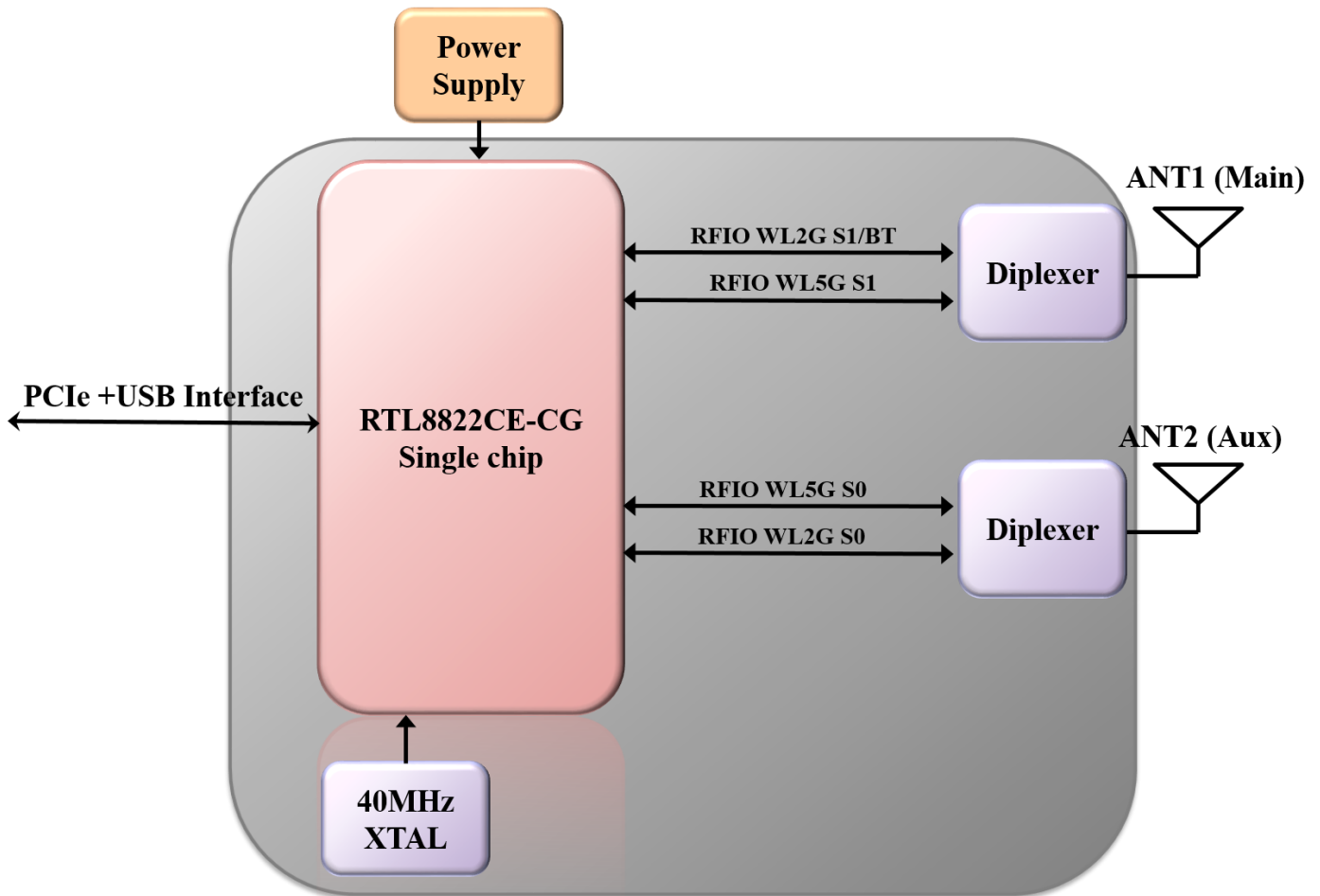
AW-CB375NF BLOCK DIAGRAM
