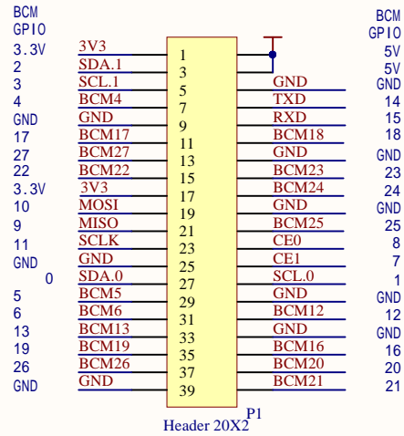
40pin connector
