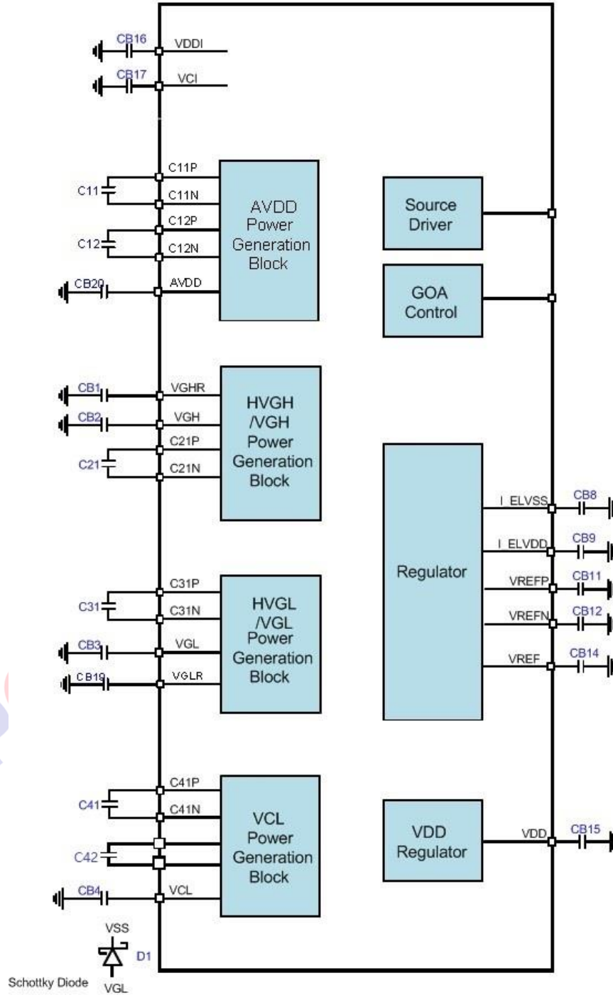
Application Ckts
