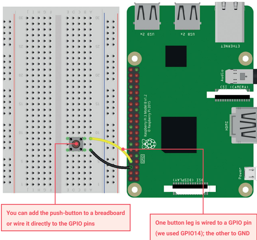
Figure 1 Connect the button
