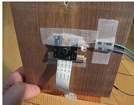
❑ Figure 6 The IR LED is taped to the underside of the roof, not too close to the camera
