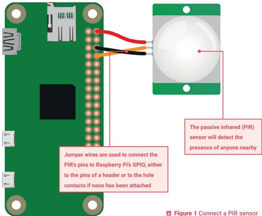
▣ Figure 1 Connect a PIR sensor
