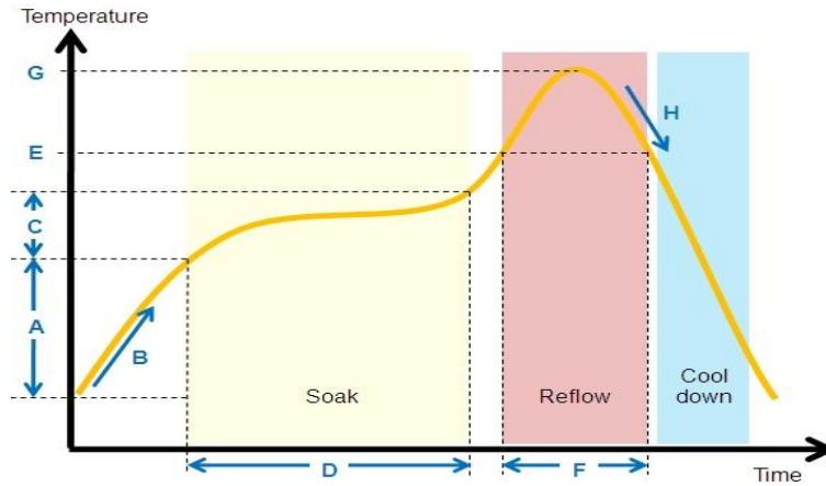
Figure 9-1 Typical Reflow Profile
