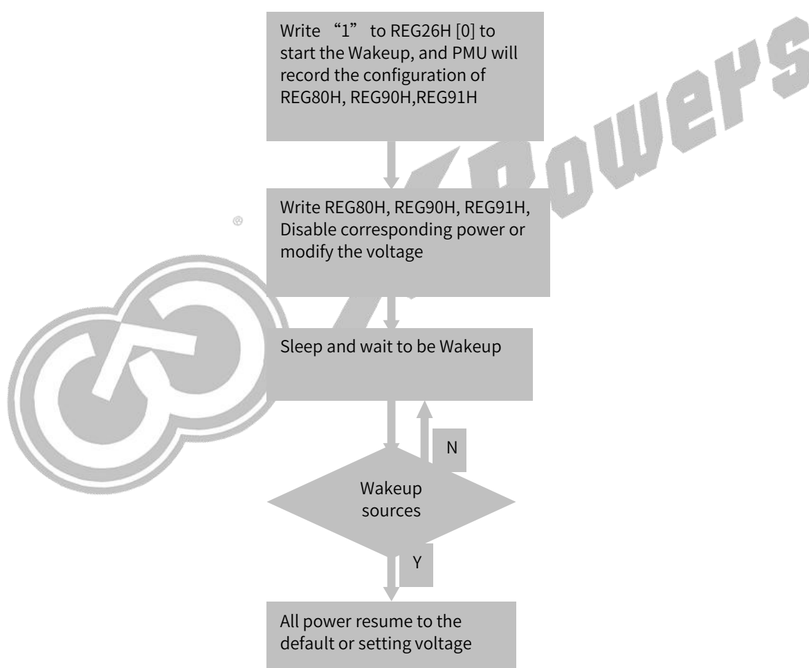
Figure 6-2 Sleep and Wakeup
