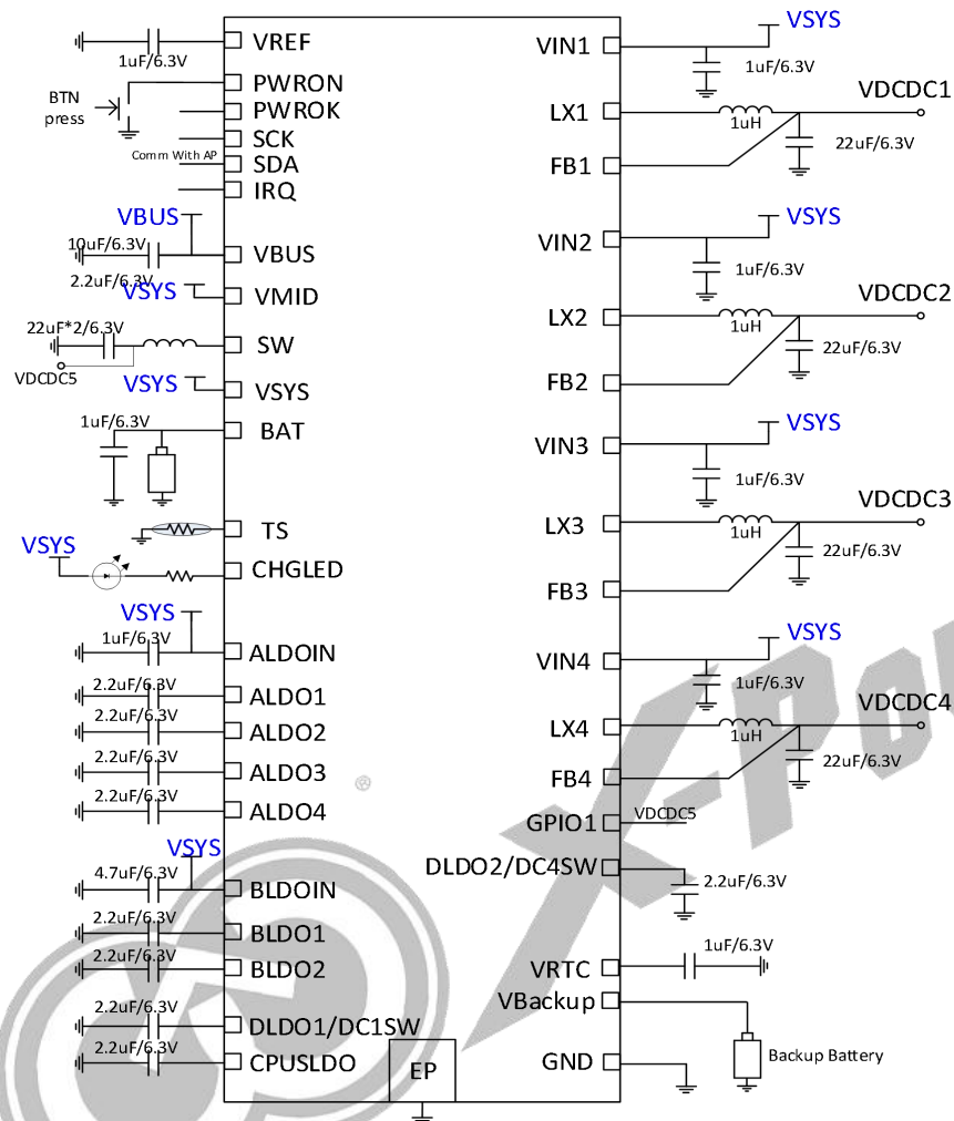
Figure 7-1 Typical Application
